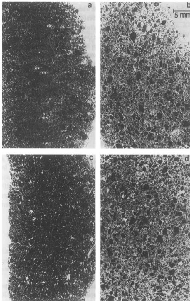
Fig. 3. Thin sections of aggregate beds of Lemnos clay loam after drying at 40°C, wetted (a) by flooding with demineralized water; (b) tension wetted with water; (c) flood wetted with \text{CaCl}_2 (10 mM); (d) tension wetted with \text{CaCl}_2 .
